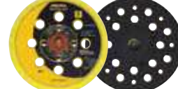
915SGV28 * 5" Backup Pad Soft, Multi-Hole, Grip 5/16 - 24 thread
